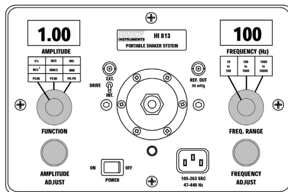
HI 813 Panel
